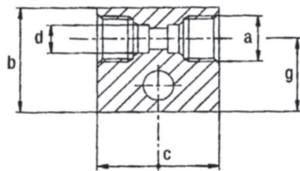
FIVE WAY WITH SCREWED SPIGOT Nº 01-4515
