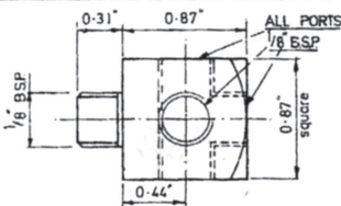
FIVE WAY WITH SCREWED SPIGOT Nº 01-4516
