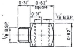
TWO WAY WITH SCREWED SPIGOT Nº 01-4517
