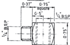
TWO WAY WITH SCREWED SPIGOT Nº 01-4518
